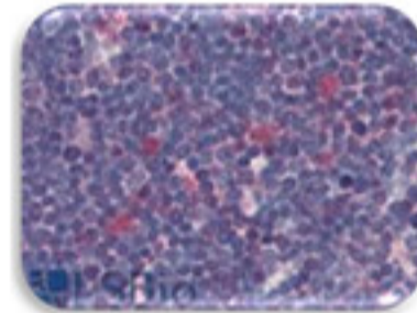
IHC analysis of CDK1 in human thymus tissue.
